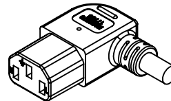
CCC FEMALE POWER PLUG PRODUCT CODE NUMBER: 17755 C-13 90 EXIT RIGHT
